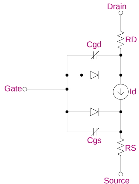
JFET Model
