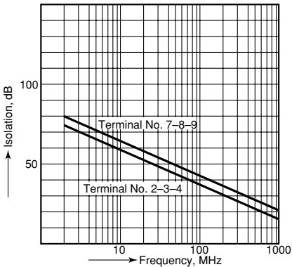
15-(1). High-frequency characteristics
