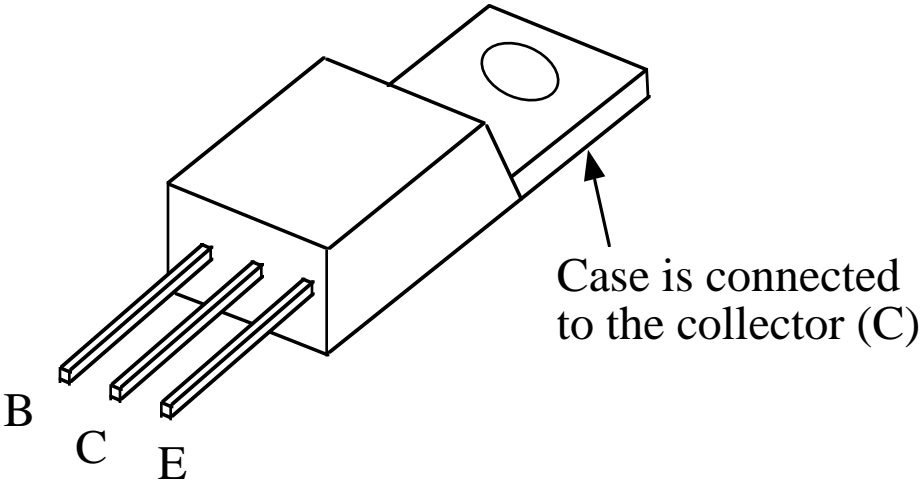
TO-220
