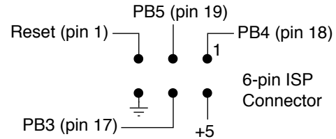
Figure 3: Top view of connections to the 6-pin ISP header
