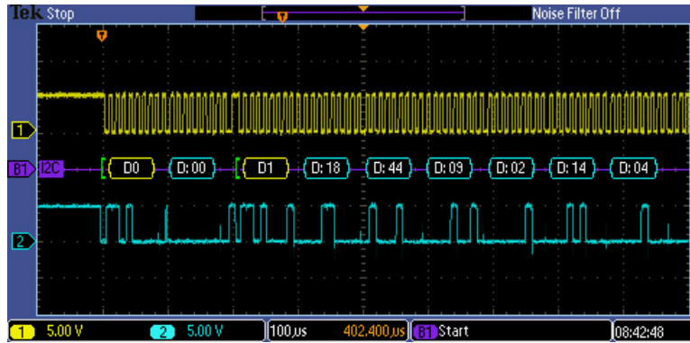
Figure 11: Tektronix I 2 C signal display
