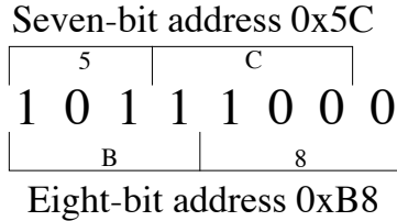
Figure 2: 7-bit and 8-bit I 2 C addresses
