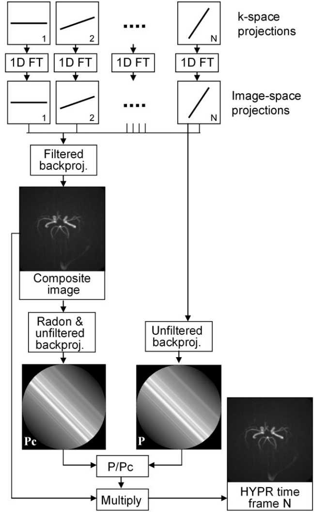
FIG. 1. Schematic diagram of the HYPR reconstruction algorithm. For simplicity, the diagram shows a single projection for each time frame. A 1D Fourier Transform converts the radial k -space lines to projections in image space. A composite image is reconstructed from the projections in all time frames. For each individual HYPR time frame, the composite image is multiplied by the unfiltered backprojected profile P specific to the time frame normalized by the corresponding unfiltered backprojected profile P_c calculated from the composite image.
