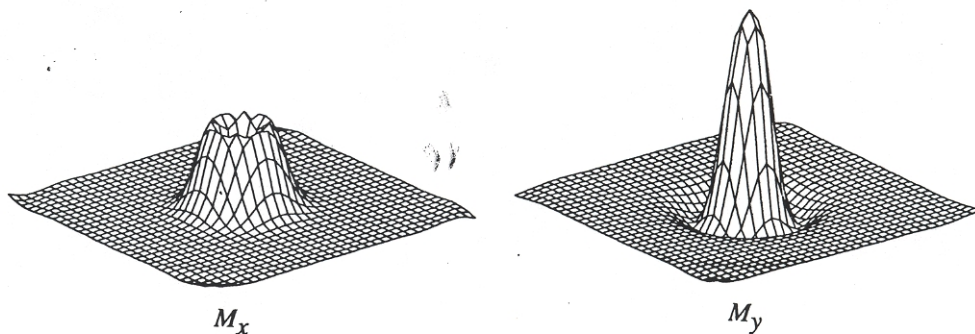
FIG. 12. Selective volume resulting from the same excitation as in Fig. 11, but with a half cycle off-resonance shift over the duration of the pulse. This corresponds to a 1 ppm shift for an 8 ms excitation pulse at 1.5 T. We have assumed the volume has been refocused with a 180^\circ pulse. The M_y component is relatively unaffected from Fig. 11. The principal effect is a nonzero M_x representing some loss in resolution and imperfect phase coherence across the volume.
