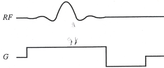
FIG. 1. Conventional slice-selective excitation. A constant slice-select gradient is applied while the RF waveform is played out. At the end of the RF the gradient is reversed to refocus the selected slice. The area of the refocusing lobe is one-half the area of the slice-select lobe in the small-tip-angle case.
