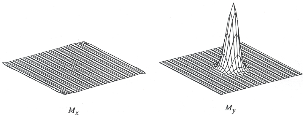
FIG. 10. Surface plots of the selective volume produced gradient waveform in Fig. 8 with the RF waveform in Fig. 9. The RF is scaled to produce a tip angle of 30^\circ . The left plot is M_x , and the right plot is M_y . Note that virtually all of the transverse magnetization is in M_y , meaning the selected volume is very well refocused. Also the sidelobes are very low.
