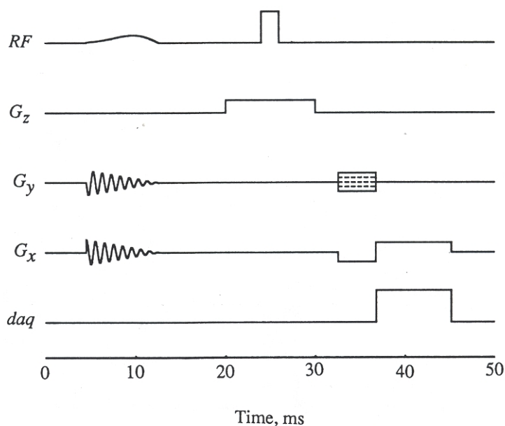
FIG. 13. Pulse sequence used to demonstrate the two-dimensional selective excitation pulse. The two-dimensional pulse is applied along the x and y axes exciting a cylinder along the z axis. A selective 180^\circ forms a spin echo of a slice of this cylinder. The resulting disk is then imaged with a conventional spin-warp pulse sequence.
